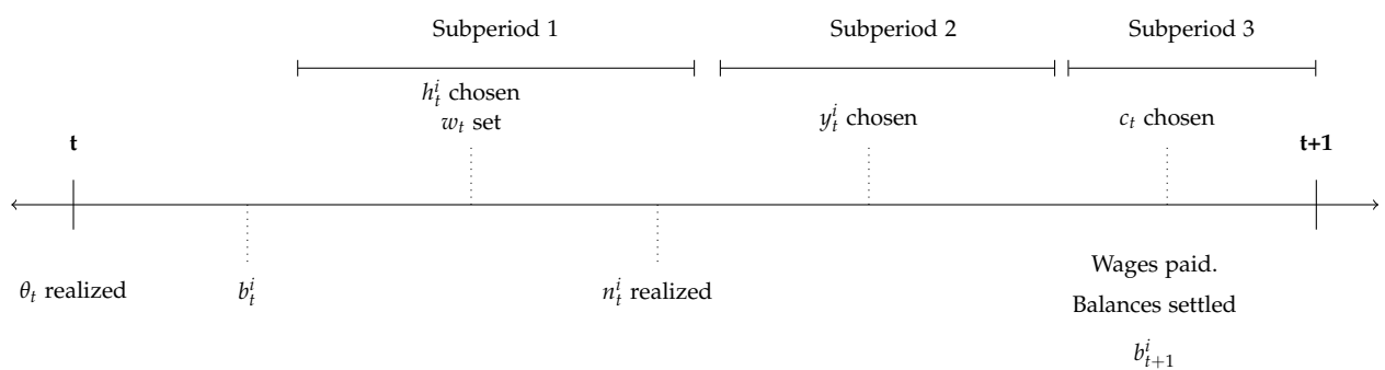
Figure 4: Model's Timing
